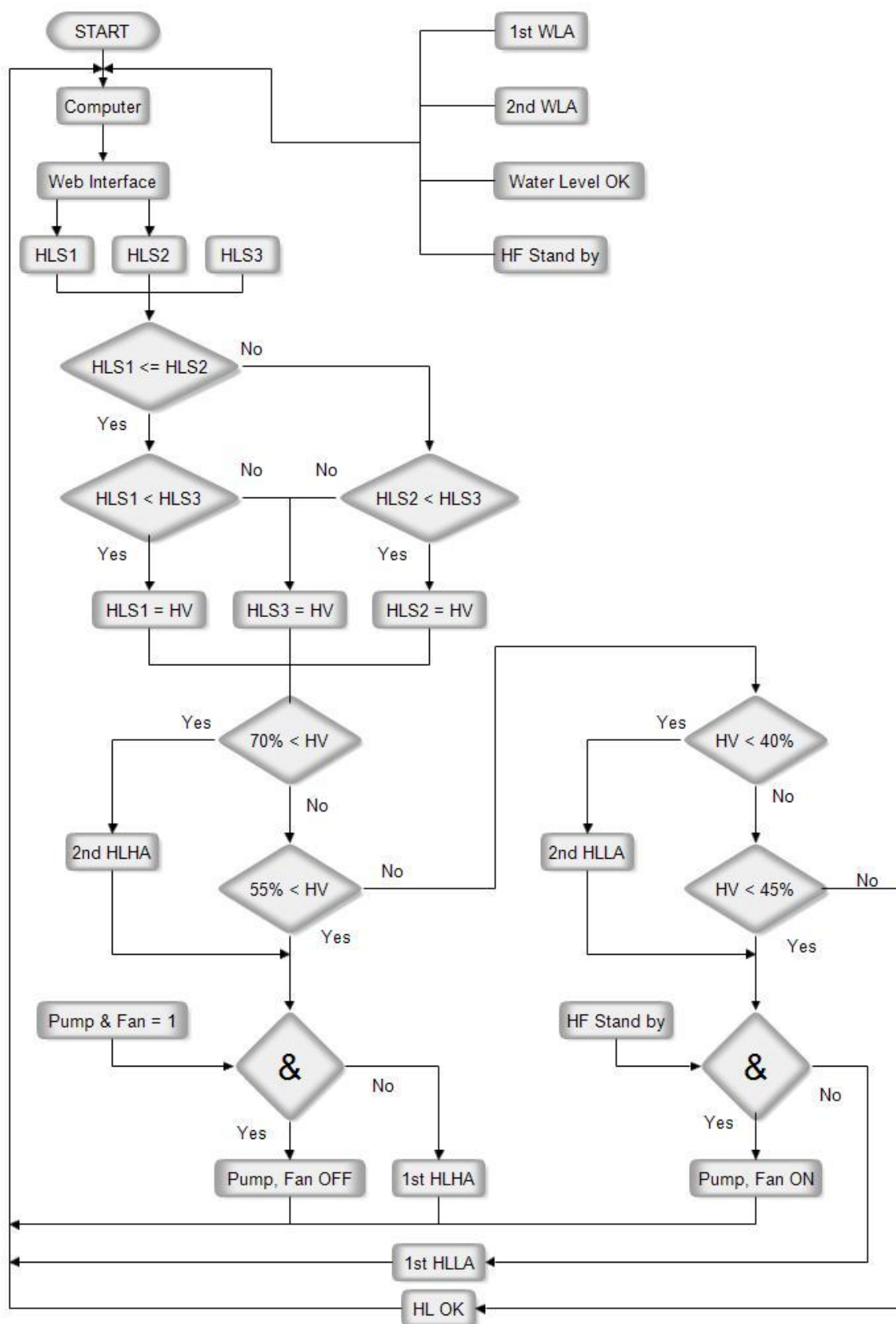
Fig , 4. Flowchart
